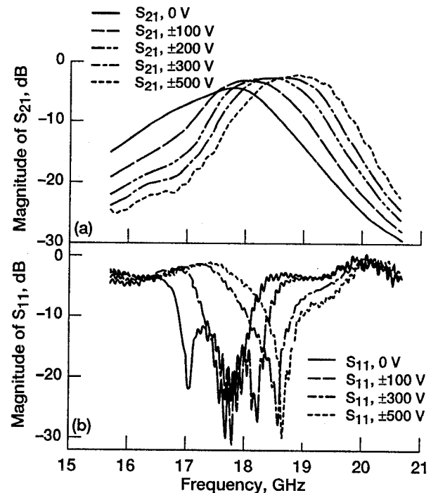
Figure 4: Field dependence of S_{21} and S_{11} for a tunable bandpass filter at 77K.
