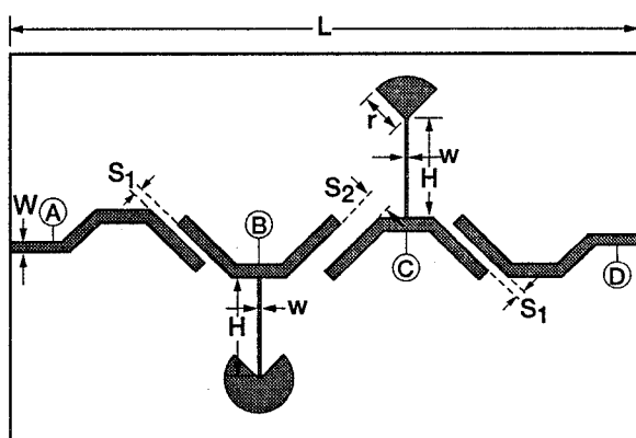
Figure 2: The geometry of the optimized tunable filter circuit. The dimensions are: W=86.25\ \mu\text{m} , L=6.8\ \text{mm} , S_1=100\ \mu\text{m} , S_2=300\ \mu\text{m} , H=1.33\ \text{mm} , w=12.5\ \mu\text{m} and r=200\ \mu\text{m} .
